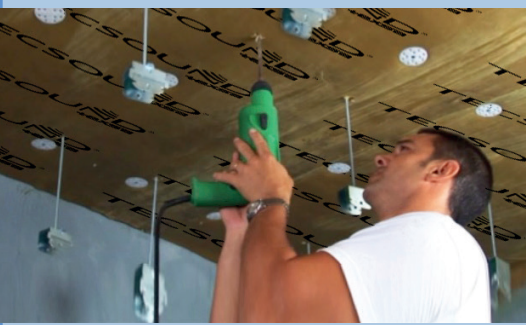
TECSOUND® 2 FT
